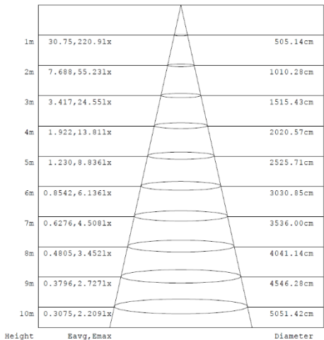
Diagram for RVC4K1in 4000K. Other diagrams available on request
